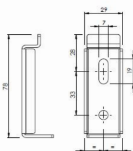
Wall support
